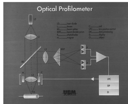
Fig.1 Optical measuring principle of the laser focus and microfocus sensors
